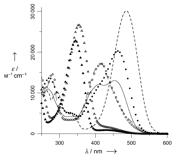
Figure 2. Absorption spectra of 1–4 in various solvents: 1 (▲) and 3 (△) in acetonitrile, 2 in acetonitrile (—) and chloroform (●), 4 in acetonitrile (---) and chloroform (○), 4H + in acetonitrile (----).
