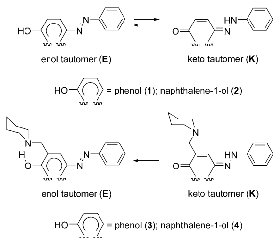
Scheme 2. Tautomeric equilibria in compounds 1–4.
